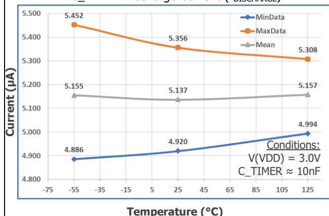
C_TIMER Discharge Current ( I_{DISCHARGE} )
