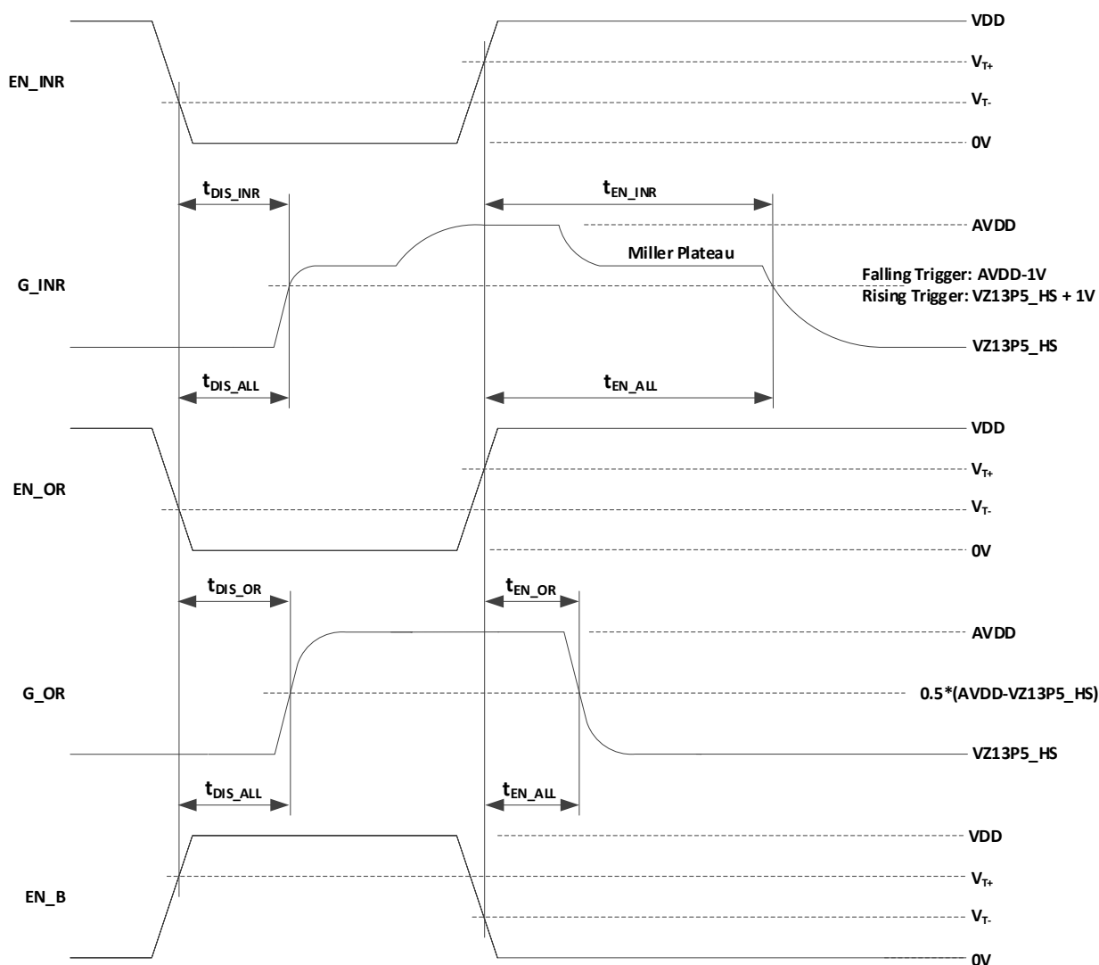
Figure 11-4. Commanded Enable and Disable Timing Diagram
