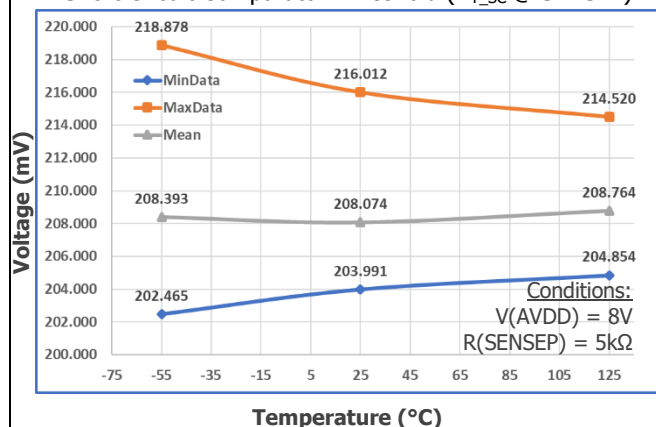
Short Circuit Comparator Threshold ( V_{T\_SC} @ SENSEP )
