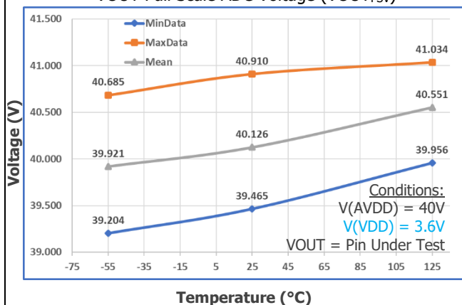
VOUT Full Scale ADC Voltage (VOUT FSV )
