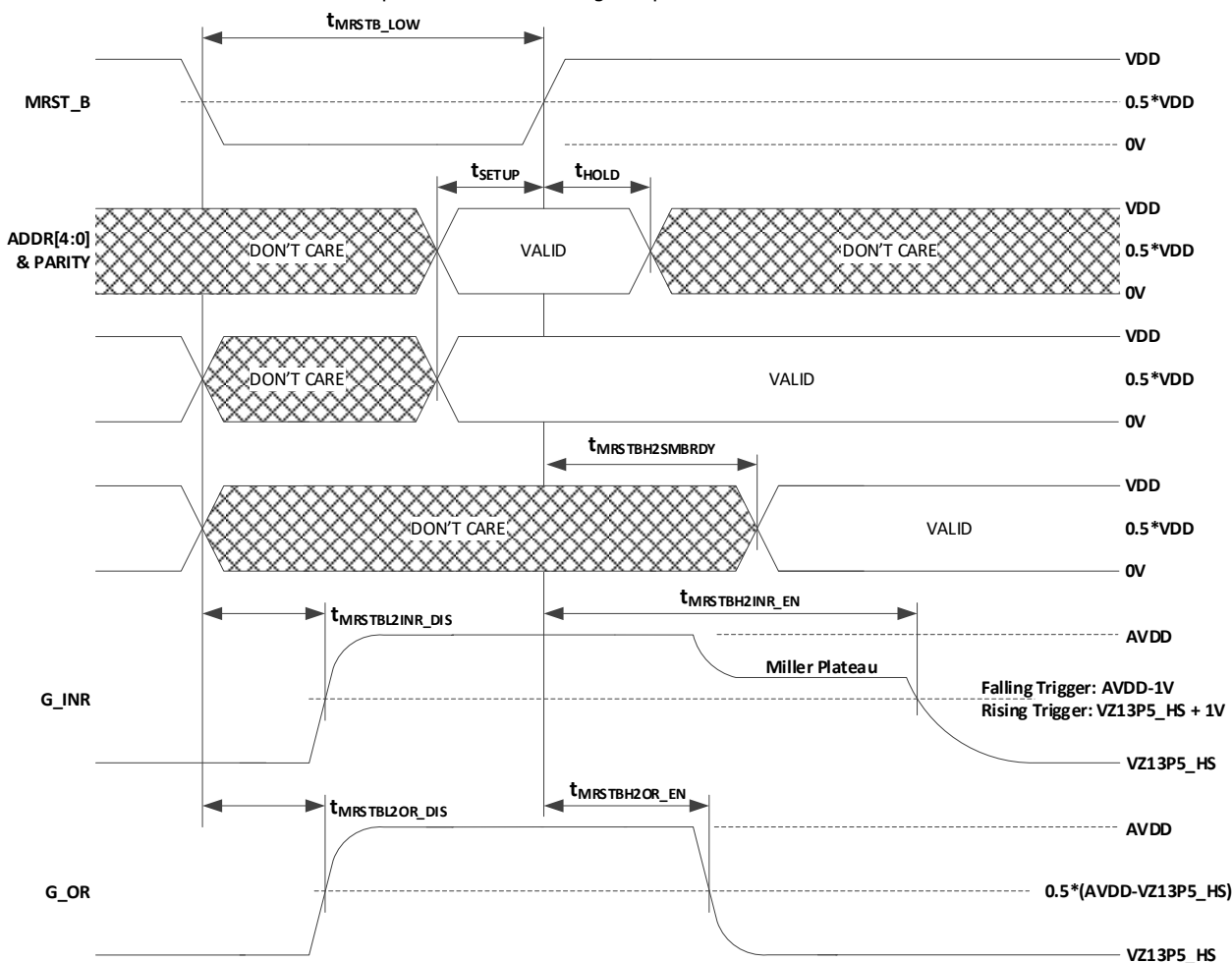
Figure 11-6. Master Reset Timing Diagram
