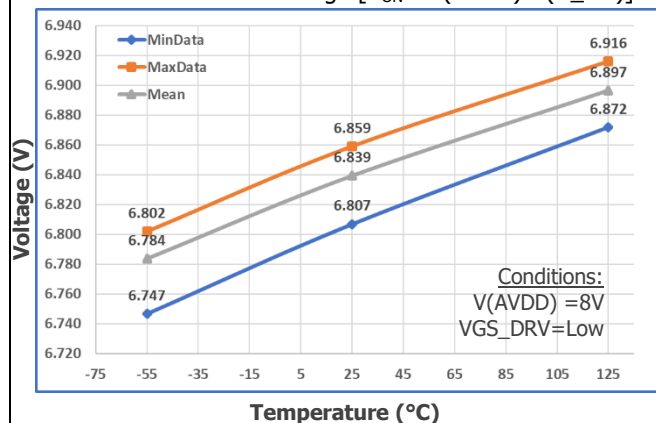
OR Gate Driver ON Voltage [ V_{ON} = V(AVDD) - V(G\_OR) ]
