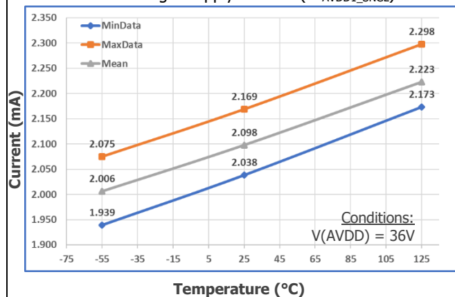
Active Single Supply Current ( I_{AVDD1\_SNGL} )
