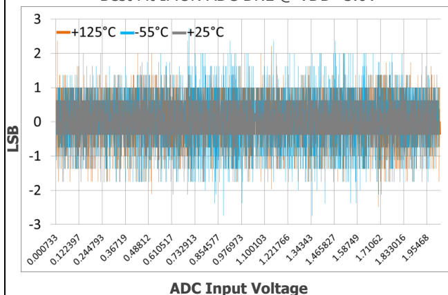
Best Fit IMON ADC DNL @ VDD=3.0V
