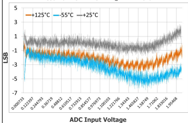
Best Fit IMON ADC INL @ VDD =3.6V
