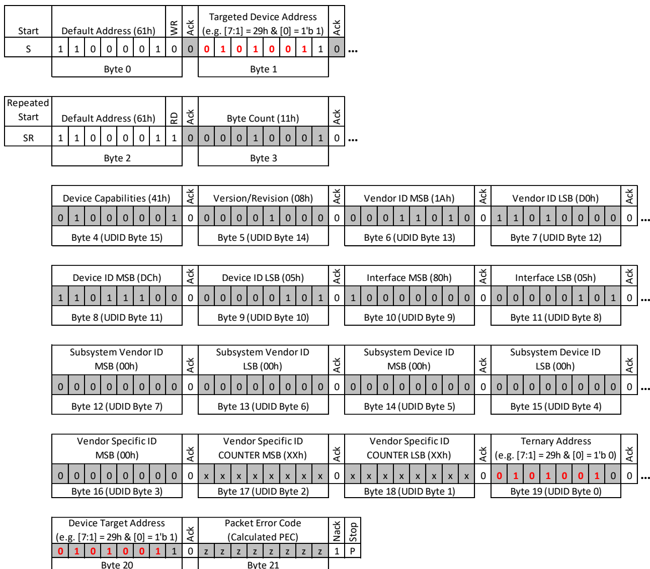
Figure 13-8. ARP DIRECTED GET UDID Command with SPSC Ternary Address 29h (41 decimal)
