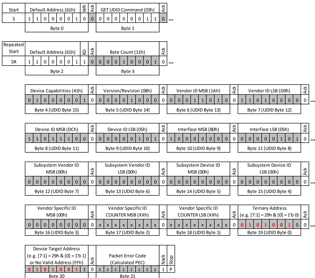
Figure 13-7. ARP GENERAL GET UDID Command with SPSC Ternary Address 29h (41 decimal)
