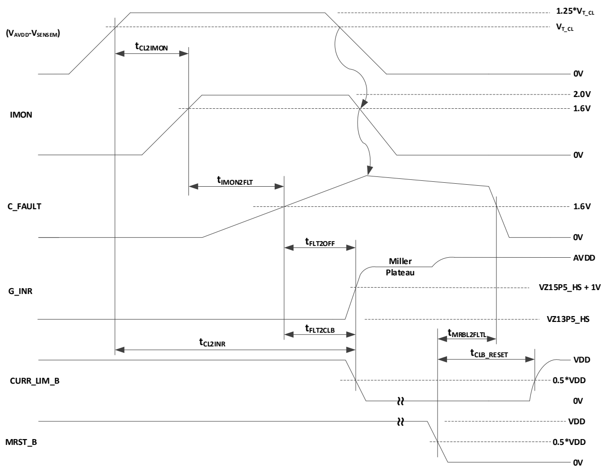
Figure 11-1. Current Limit Response Timing Diagram
