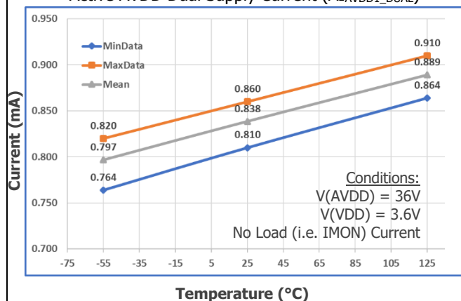
Active AVDD Dual Supply Current ( I_{AVDD1\_DUAL} )
