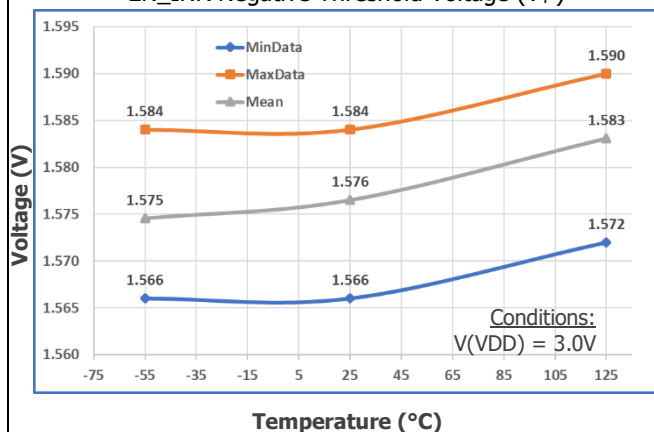
EN_INR Negative Threshold Voltage ( V_{T-} )
