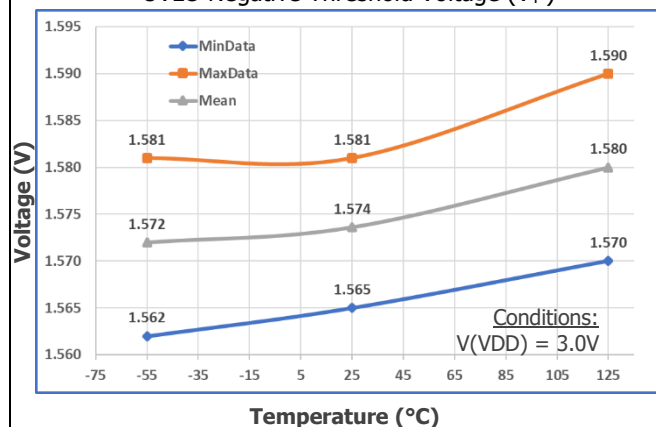
UVLO Negative Threshold Voltage ( V_{T-} )
