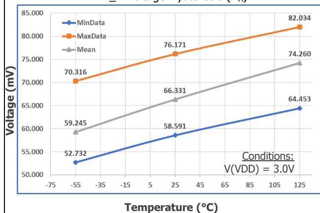
EN_B Voltage Hysteresis ( V_H )
