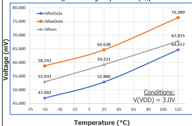
EN_INR Voltage Hysteresis ( V_H )
