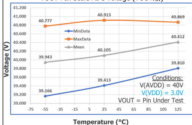
VOUT Full Scale ADC Voltage (VOUT FSV )
