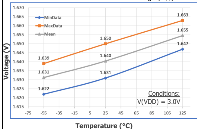
FEEDBACK Positive Threshold Voltage ( V_{T+} )
