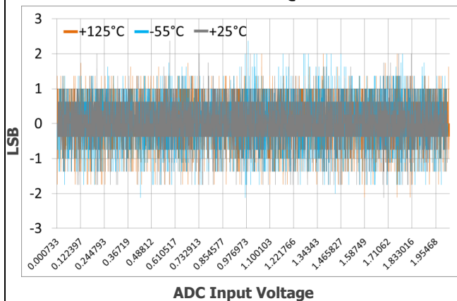
Best Fit IMON ADC DNL @ VDD=3.3V
