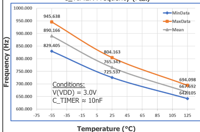
C_TIMER Frequency ( F_{CLK} )
