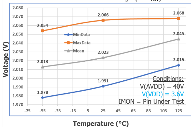
IMON Full Scale ADC Voltage (ADC FSV )
