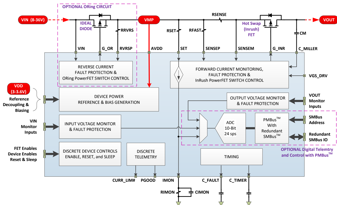
Figure 1-3-1. UT36PFD103 Block Diagram
