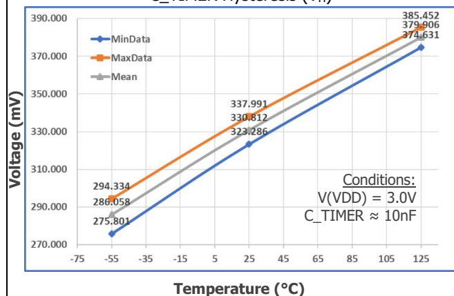
C_TIMER Hysteresis ( V_H )
