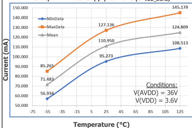
Sleep VDD Dual Supply Current ( I_{VDD\_DUAL} )
