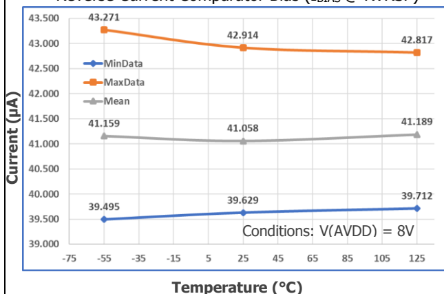
Reverse Current Comparator Bias ( I_{BIAS} @ RVRSP )
