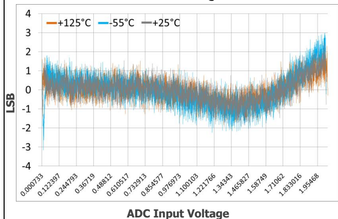
Best Fit IMON ADC INL @ VDD=3.3V
