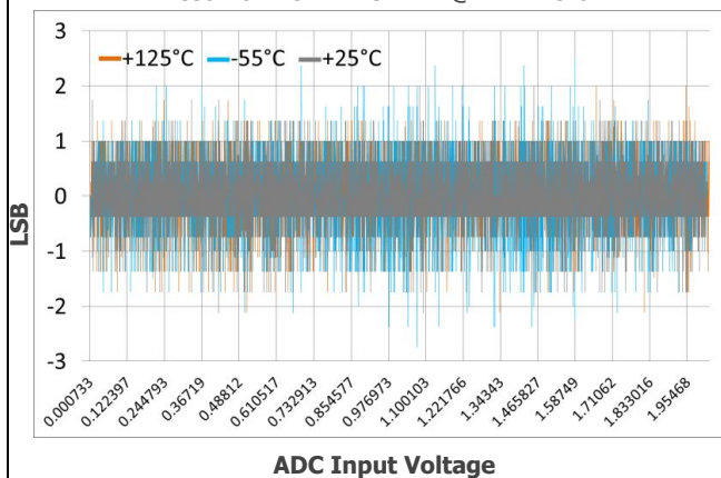
Best Fit IMON ADC DNL @ VDD=3.6V
