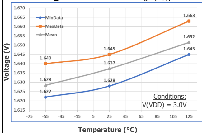
EN_B Positive Threshold Voltage ( V_{T+} )
