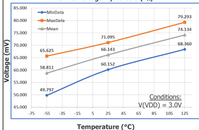
UVLO Voltage Hysteresis ( V_H )
