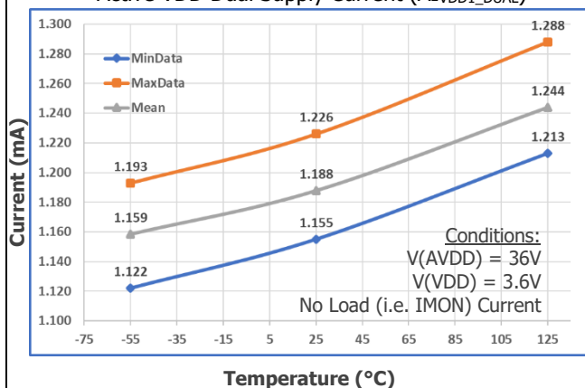
Active VDD Dual Supply Current ( I_{VDD1\_DUAL} )
