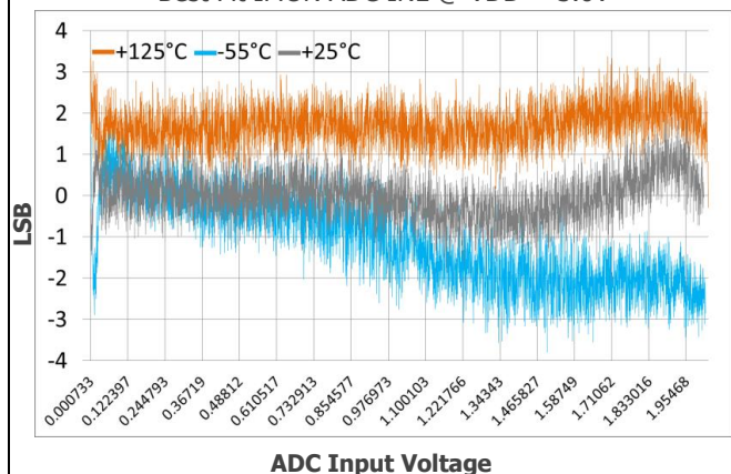
Best Fit IMON ADC INL @ VDD = 3.0V
