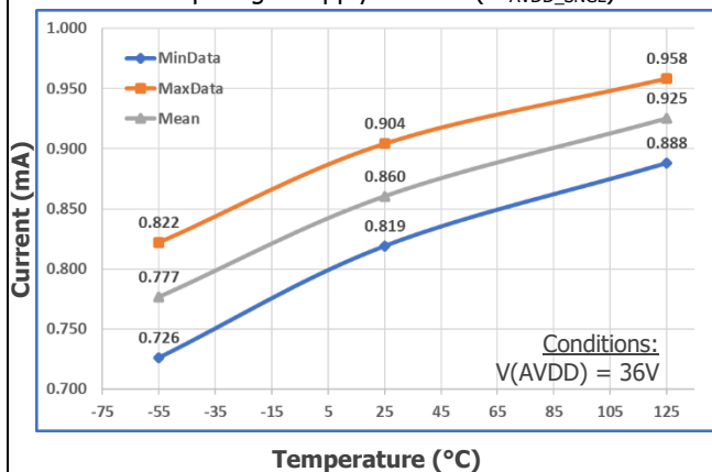
Sleep Single Supply Current ( I_{AVDD\_SNGL} )
