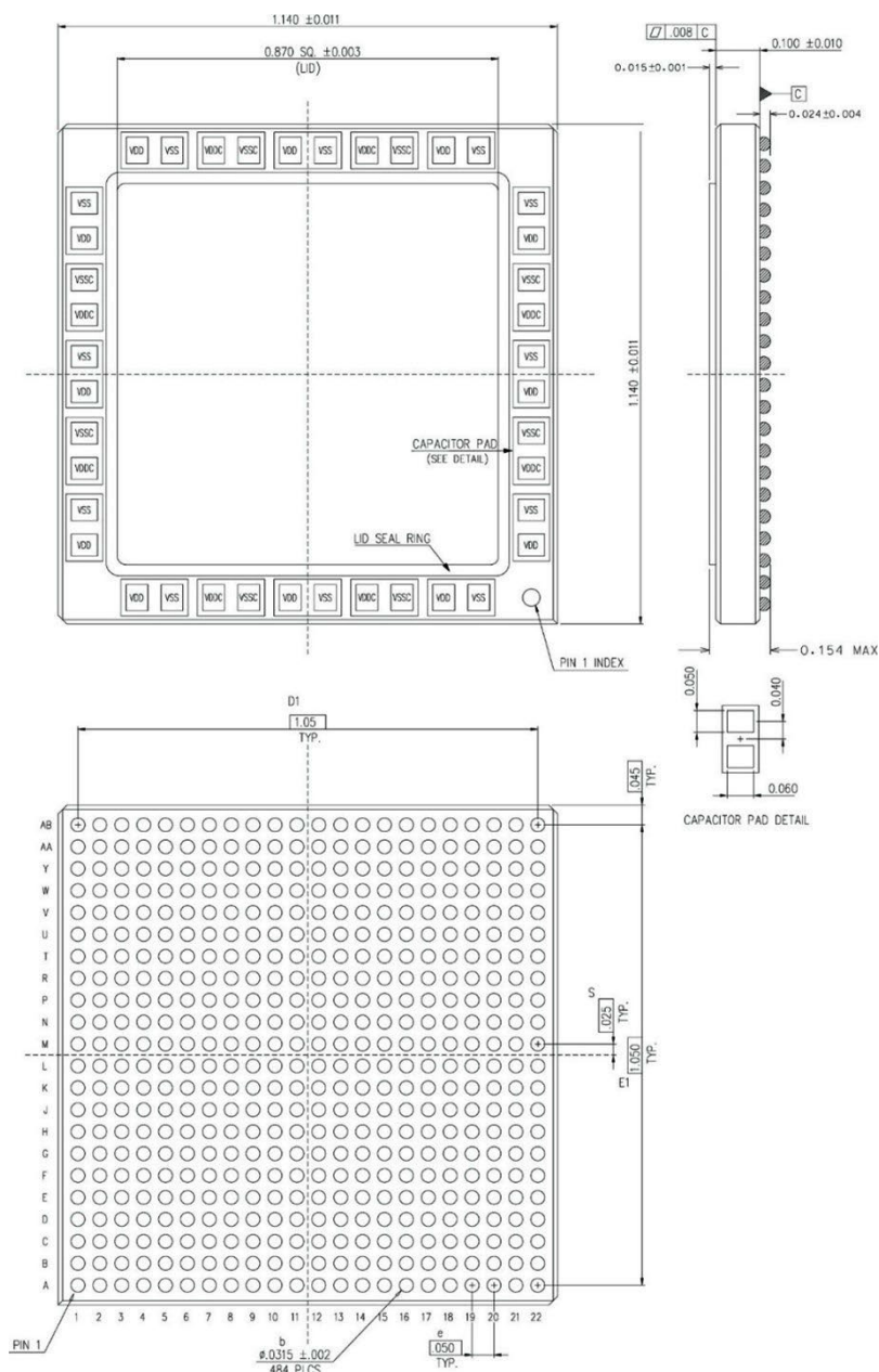
Figure 18. 484-lead Ceramic Column Grid Array
