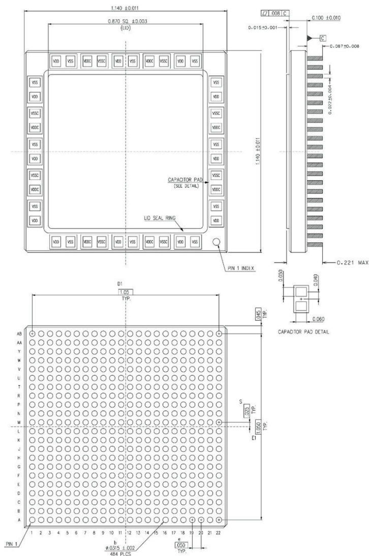
Figure 19. 484-lead Ceramic Ball Grid Array
