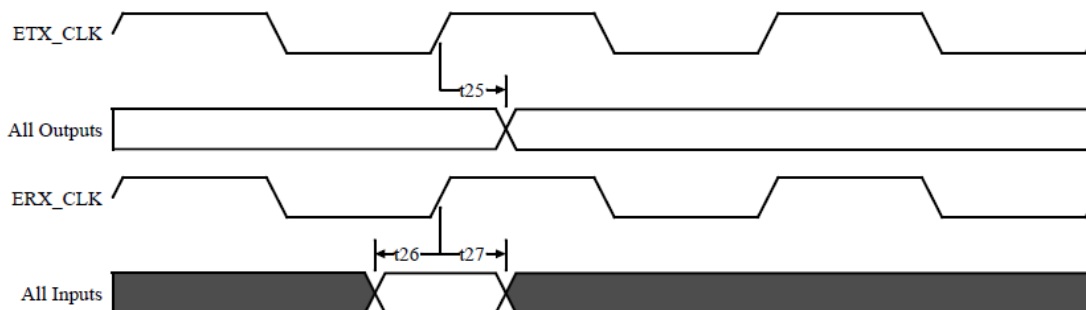
Figure 13. Ethernet Transmit and Receive Timing
