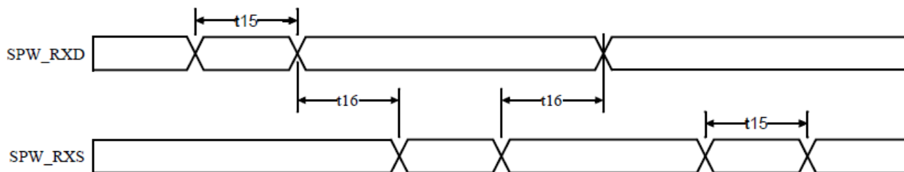
Figure 9. Space Wire Receive Timing Diagram
