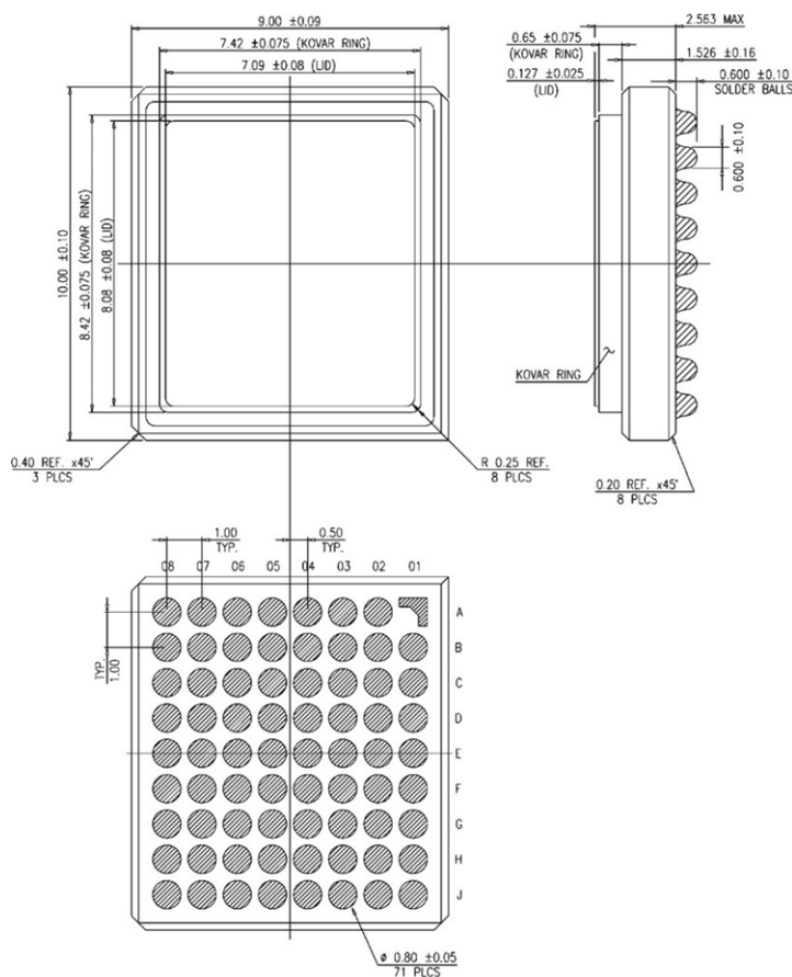
Figure 7.2: 71-Pin Ceramic Ball Grid Array (C-BGA) Package
