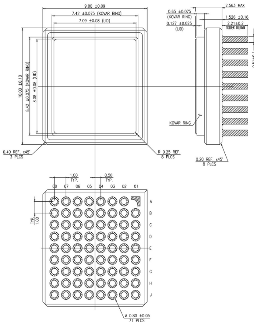
Figure 7.3: 71-Pin Ceramic Column Grid Array (C-CGA) Package
