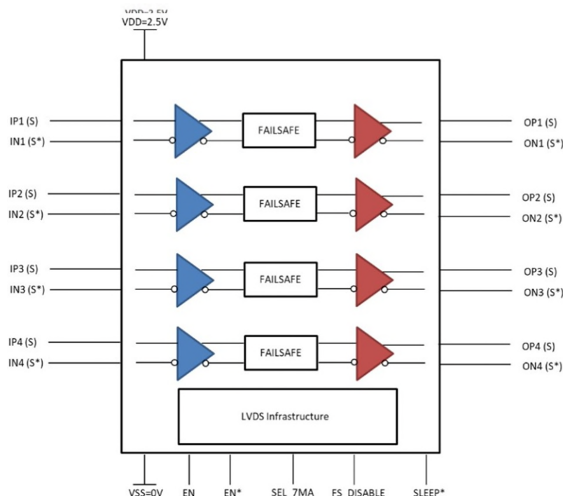
Figure 1.3: UT54LVDS454 Quad, Simplex Repeater Block Diagram
