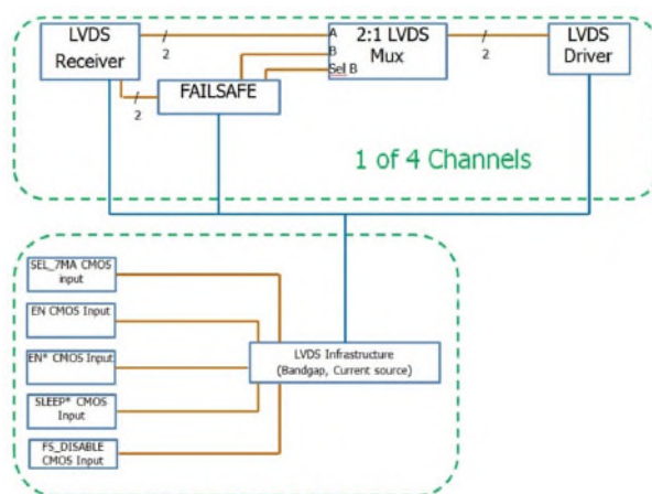
Figure 1.1: UT54LVDS454 Repeater Single Channel Functional Block Diagram
