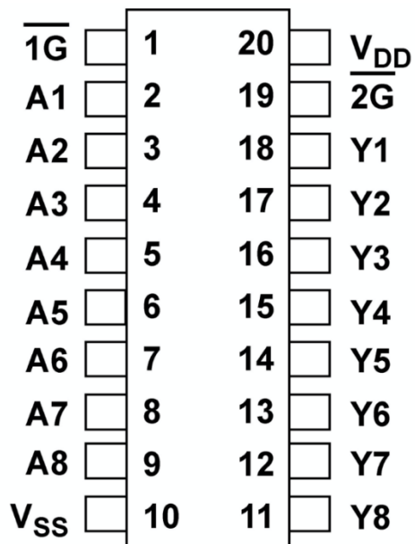
Figure 1: 20-Pin DIP Top View
