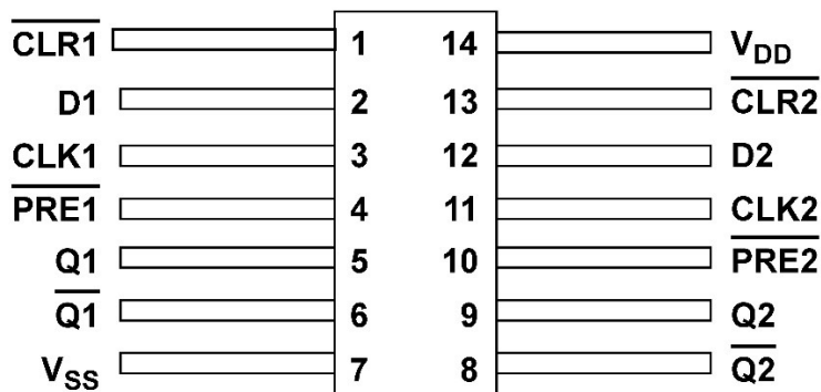
Figure 1: 14-Lead Flatpack, Top View
