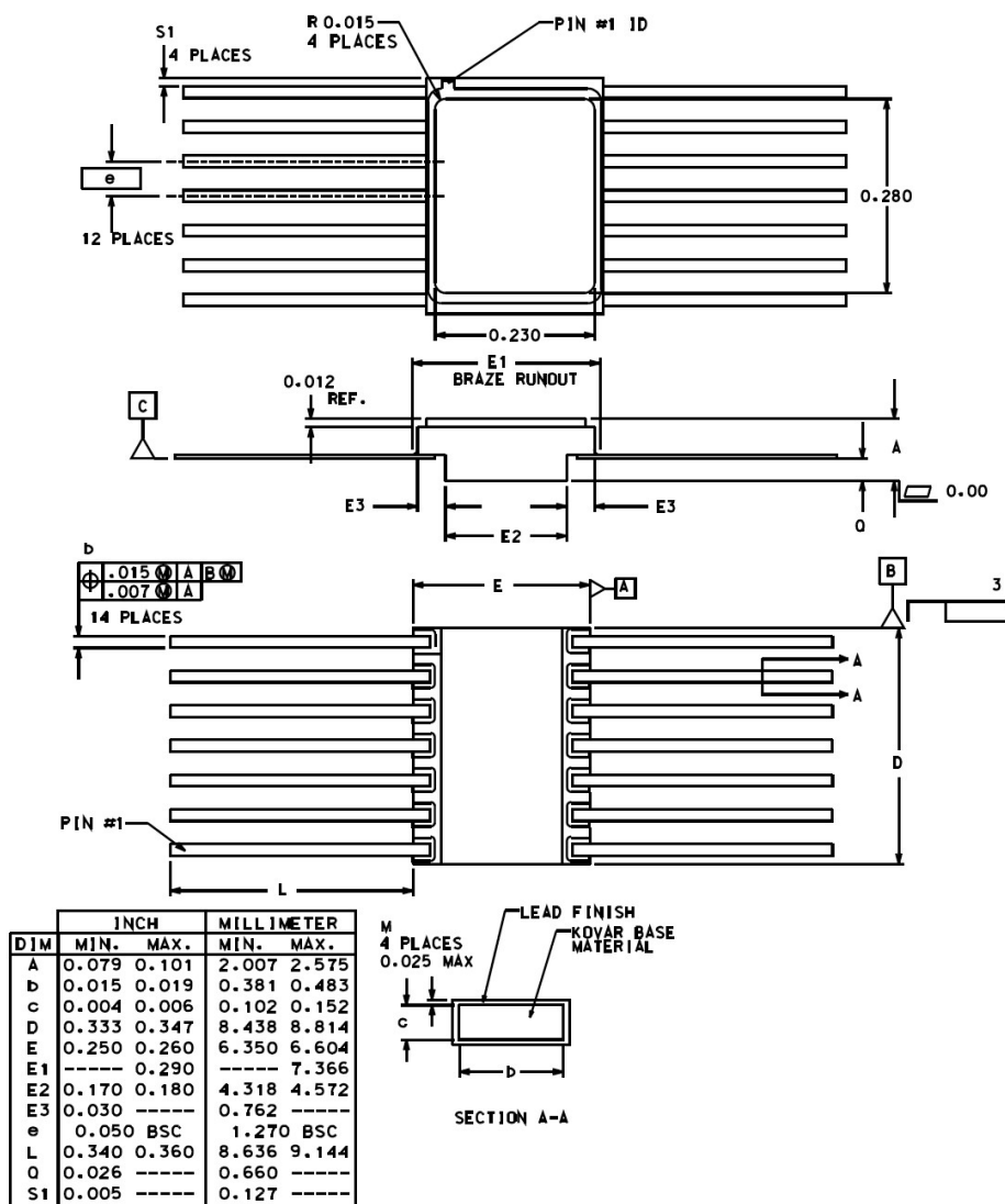
Figure 2: Figure 1. 14-lead Flatpack
