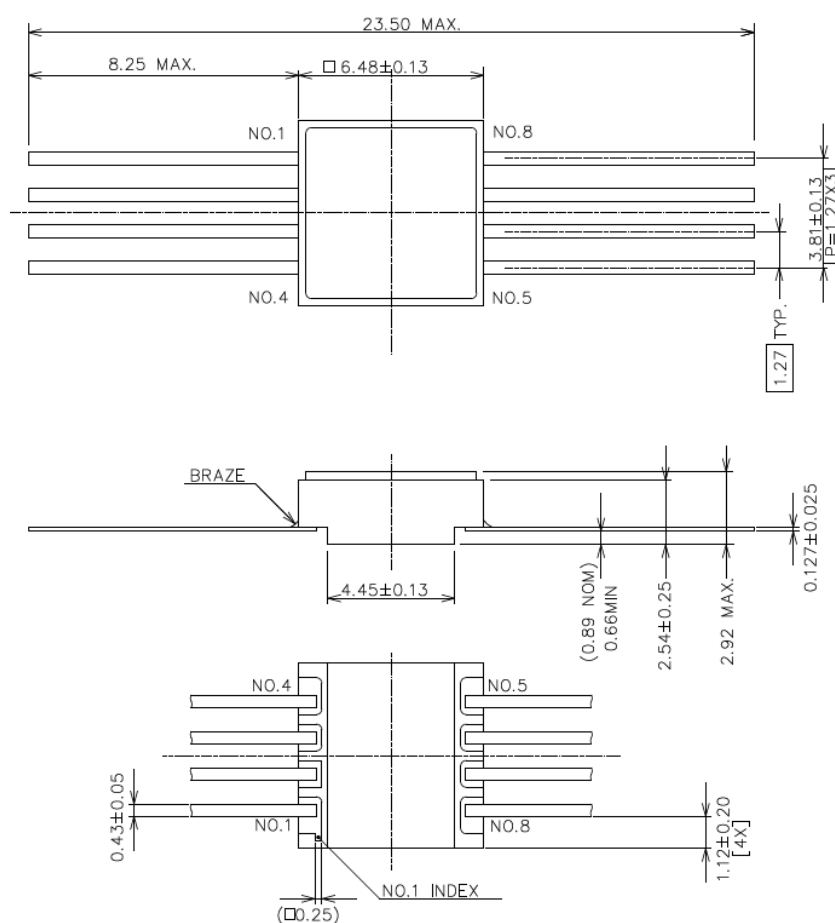
Figure 9. 8-pin Dual-In-Line Flatpack
