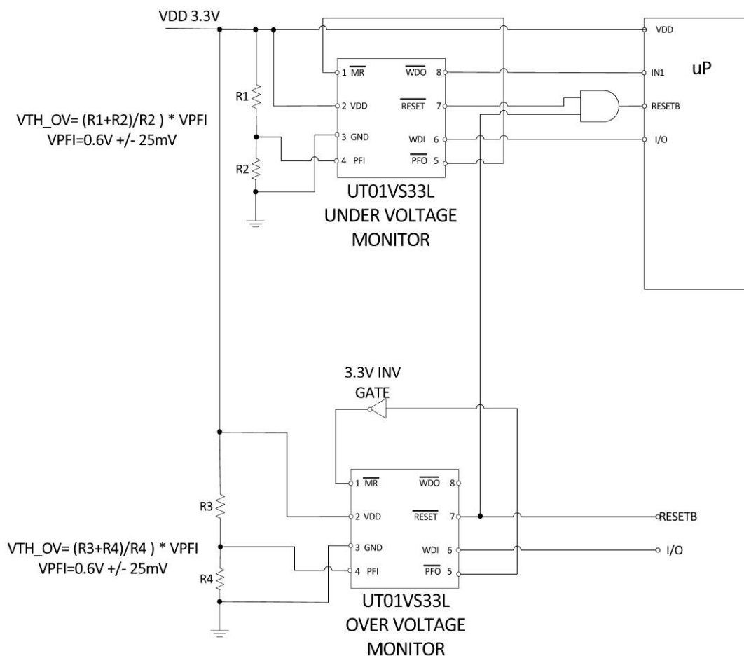
Figure 8. UT01VS33L Under Voltage and Over Voltage Power Supply Monitoring and Reset
