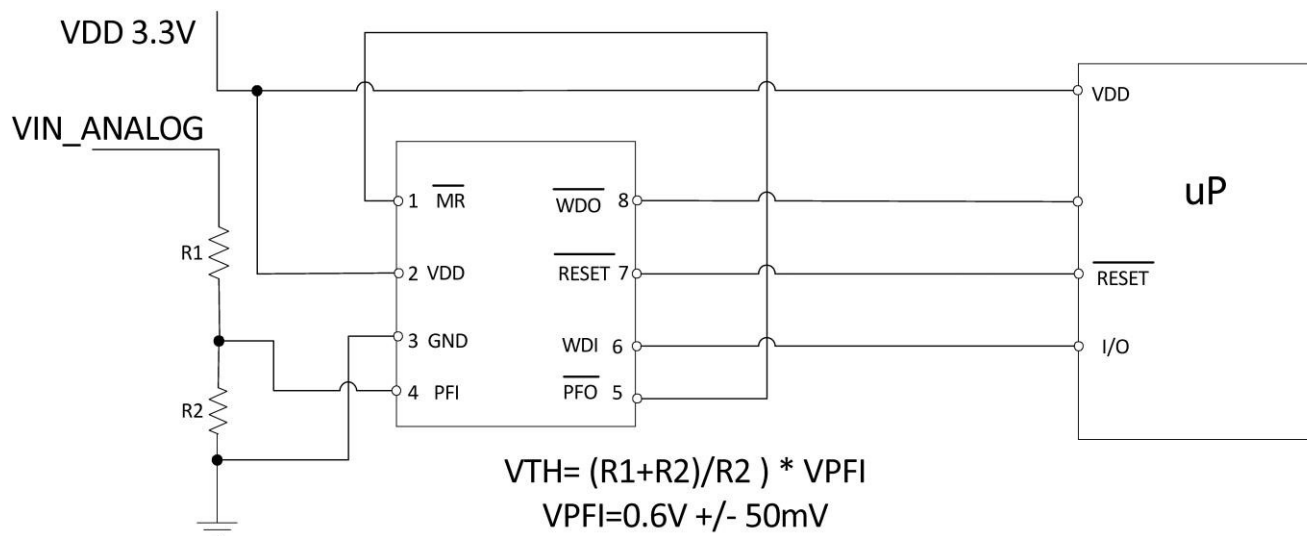
Figure 5. UT01VS33L Under Voltage Monitor and Detection
