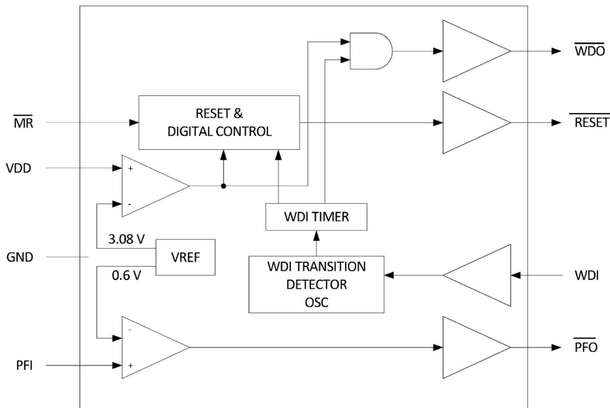
Figure 1. UT01VS33L Functional Block Diagram
