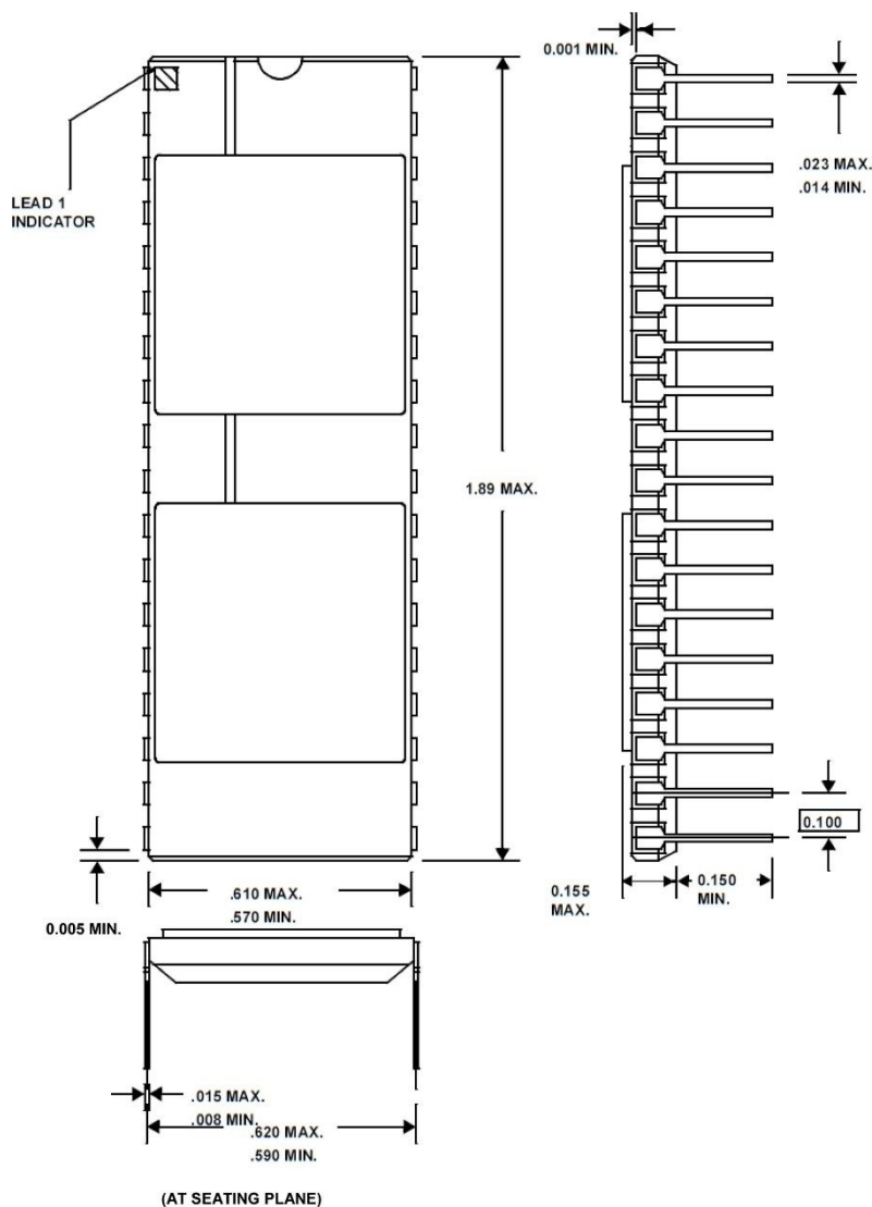
Figure 14. 36-Pin Side-Brazed DIP, Dual Cavity
