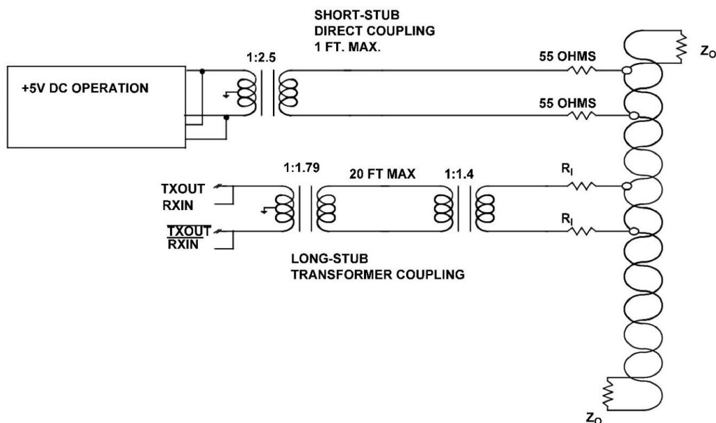
Figure 5. Bus Coupling Configuration
