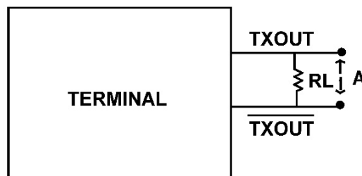
Figure 8. Transceiver Test Circuit MIL-STD-1553
