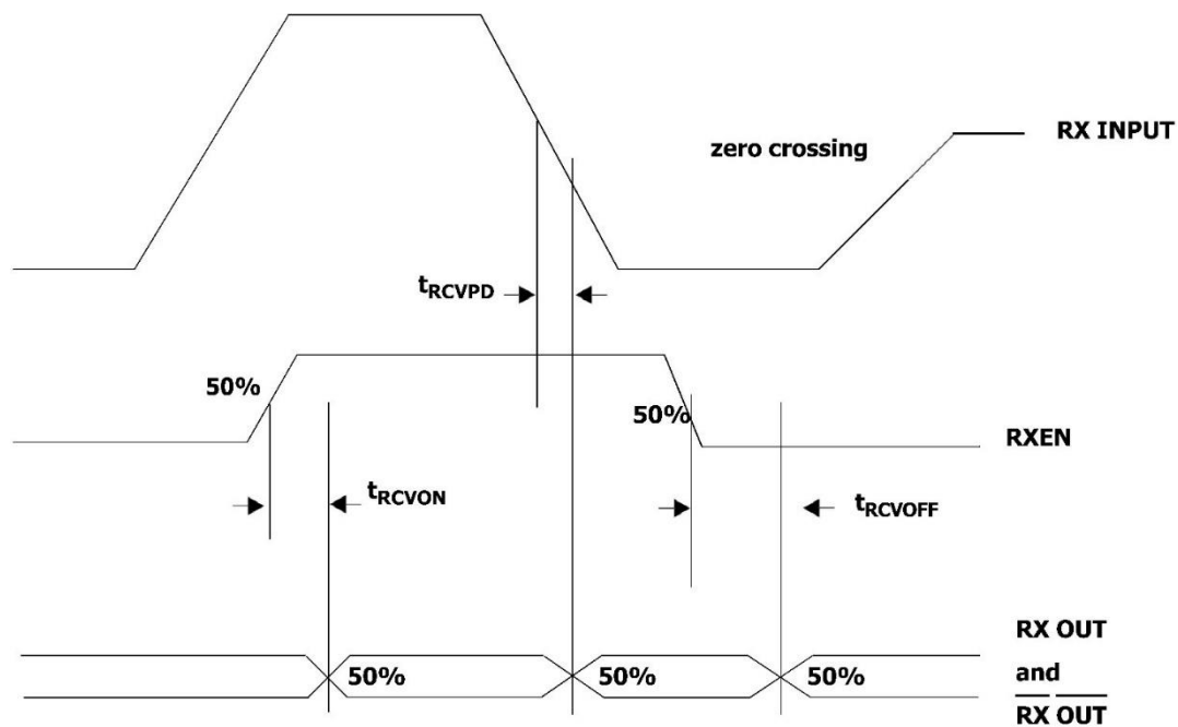
Figure 13. Receiving Timing
