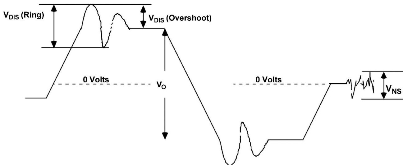
Figure 9. Transmitter Output Characteristics ( V_{DIS} , V_{NS} , V_O )
