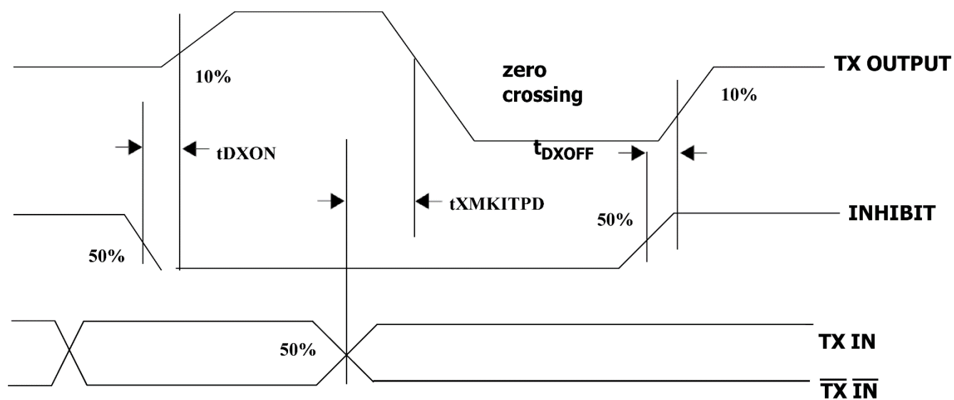
Figure 12. Transmitter Timing
